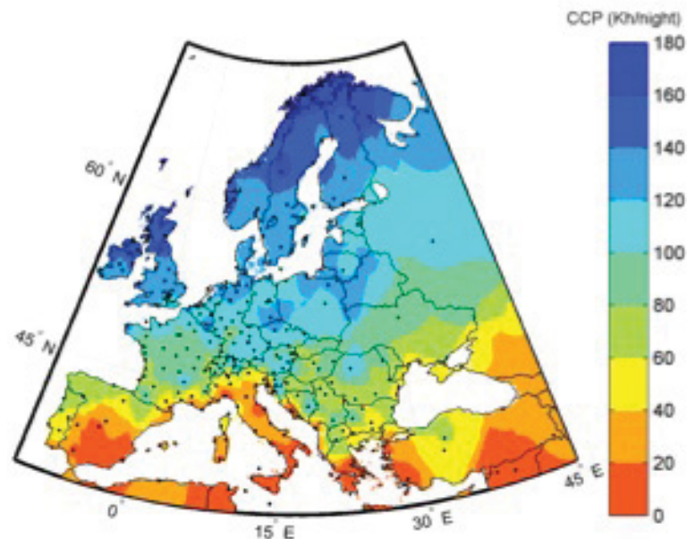
Figure 1. Map of mean climatic cooling potential (Kh/night) in July based on Meteonorm data 1 .
